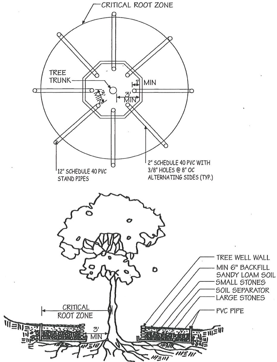
Figure E-11: Tree Well and Aeration System
