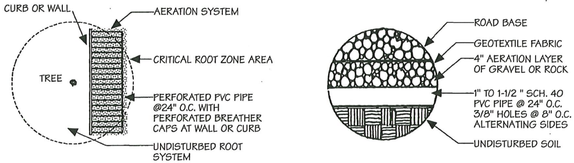
AERATION PLAN
