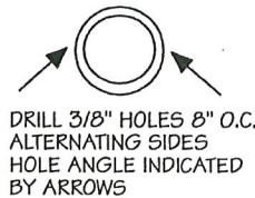
PIPE SECTION
