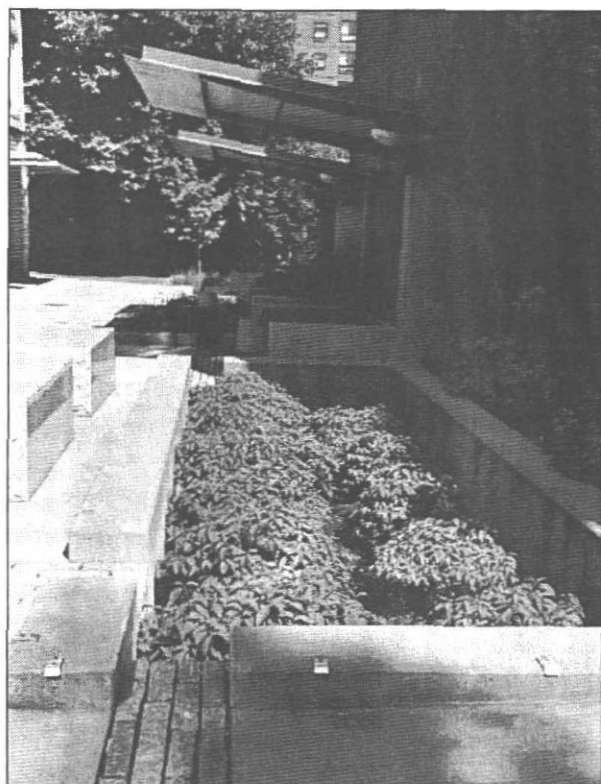
Figure 4.20. Bioretention areas can be designed attractively to suit urban stormwater management conditions.
