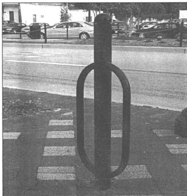
Figure 3.20. The recommended bollard for the Route 1 corridor is Bollard 35, BKR permanent mount, manufactured by Victor Stanley, Inc., or equal by another manufacturer. The bollard can also serve as a bicycle storage area.
